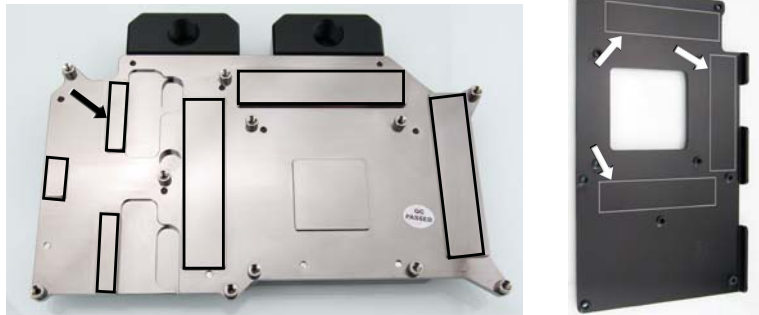
VID-NXTTN Water Block and Back Plate Thermal Pad Locations
