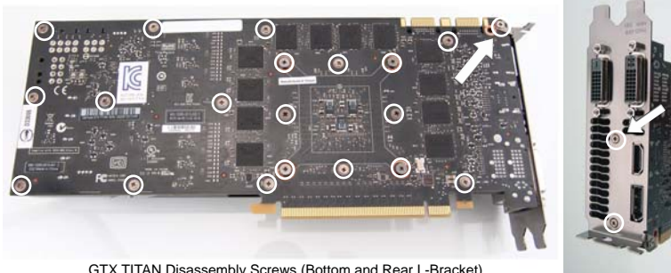
GTX TITAN Disassembly Screws (Bottom and Rear L-Bracket)
