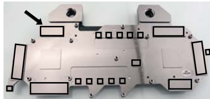
VID-NX690 Thermal Pad Locations
